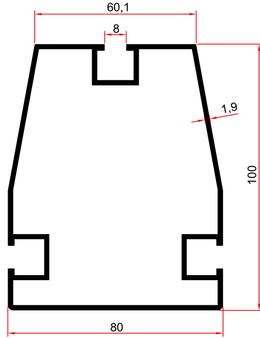
4772 2,286 Kg/m
