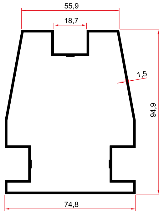
4774 1,634 Kg/m
